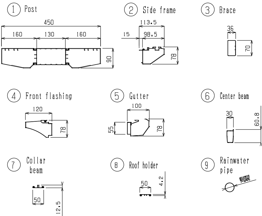
Main parts cross-section drawing(S=1/10)
